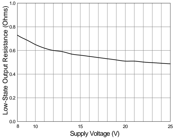
Fig. 25 Low-State Output Resistance vs. Supply Voltage
